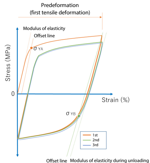
Fig. 2 Conceptual Diagram of Bauschinger Effect Evaluation Results
