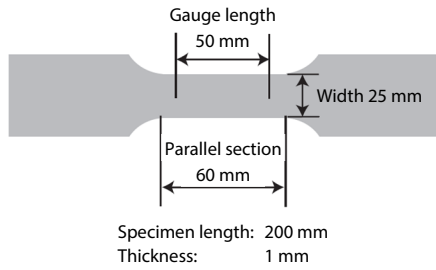
Fig. 4 Specimen Shape (as specified by JIS Z2241 No. 5)
