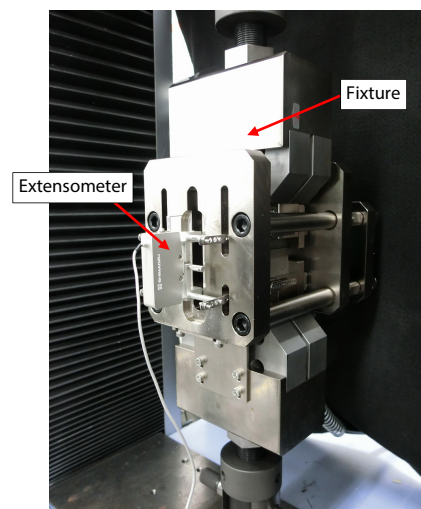
Fig. 3 Bauschinger Effect Measuring Fixture
