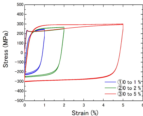
Fig. 5 Repeated Stress - Strain Curves
