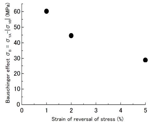
Fig. 6 Relation between Bauschinger Stress \sigma_B and Stress Reversal Strain
