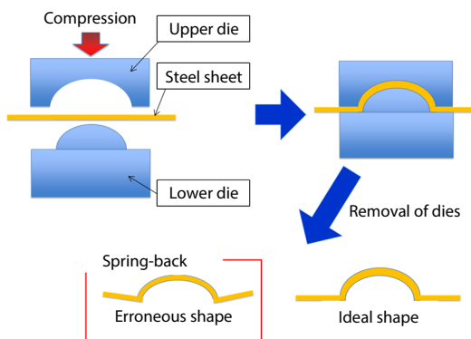
Fig. 1 Spring-back Phenomenon in Steel Sheet Forming
