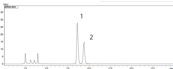
Chromatogram of Levocarnitine oral liquid
