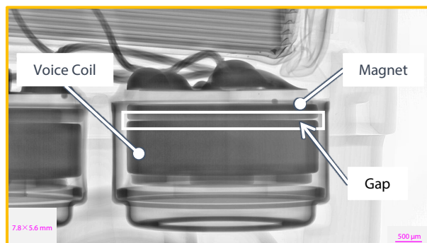
Fig. 4 X-ray Fluoroscopic Image of the Speaker
