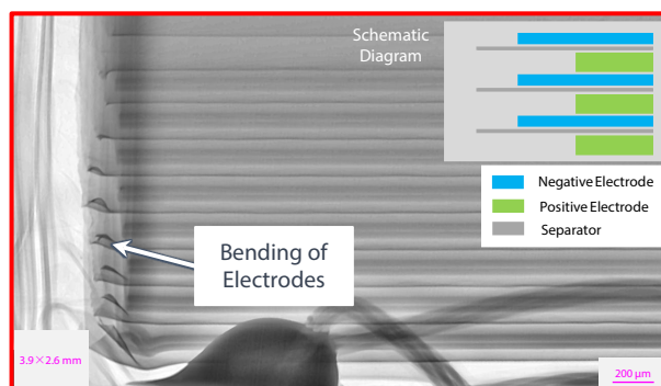
Fig. 3 X-ray Fluoroscopic Image of the Lithium-ion Battery
