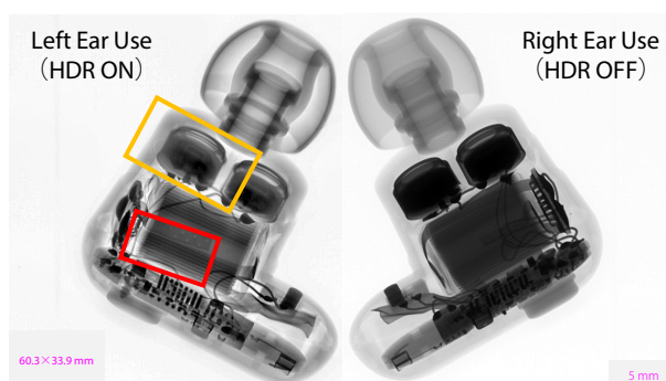
Fig. 2 X-ray Fluoroscopic Image of Wireless Earphones
