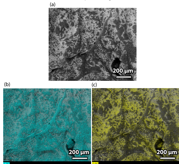
Fig. 22 Element Distribution by EDS (Crisp Sample) (a) Backscattered Electron Image, (b) Element Distribution (Carbon), (c) Element Distribution (Oxygen)
