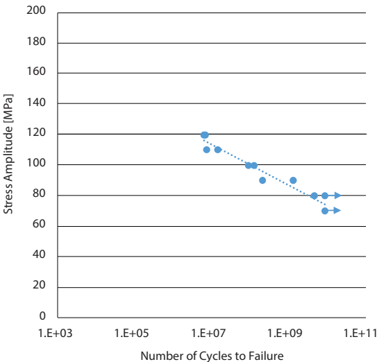
Fig. 5 S-N Diagram with A6063
