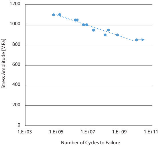
Fig. 4 S-N Diagram with SNCM439
